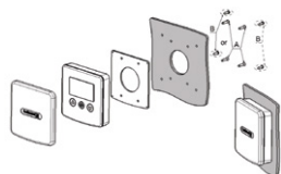
WALL MOUNTING
