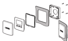
PANEL MOUNTING
